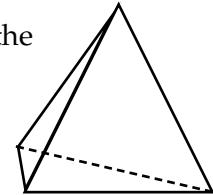
regular tetrahedron
